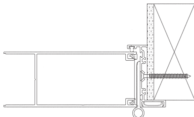
Z-bar Frame Illustration A
